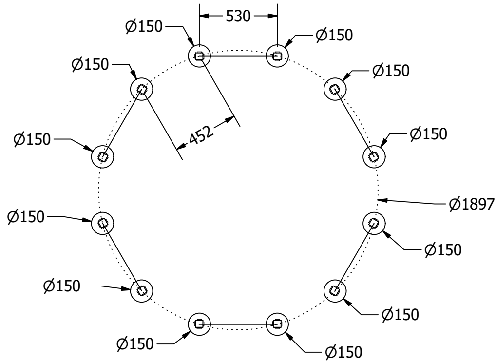
SECTION A-A SCALE 0.04
